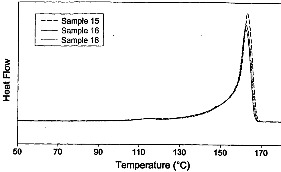
Fig. 9 DSC Melting of Plasticized Propylene Impact Copolymers
